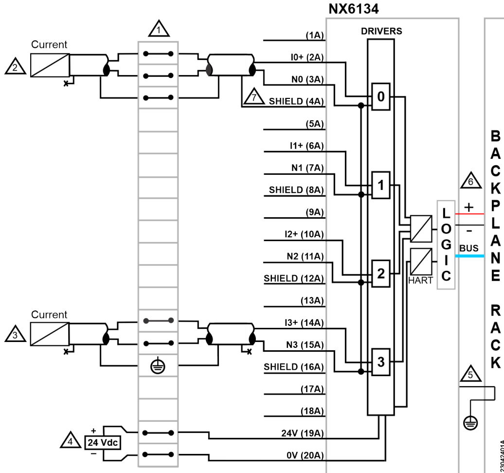
Figure 3: Electric Diagram
