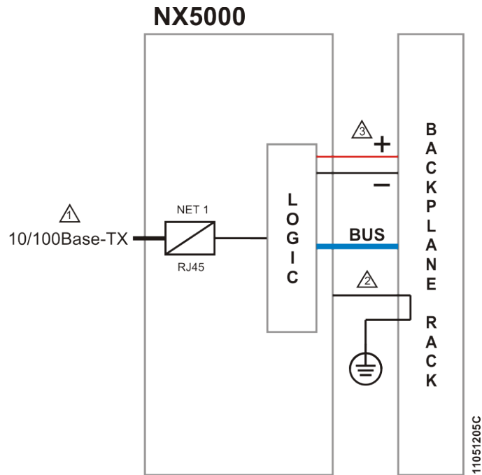
Figure 2: Electric diagram
