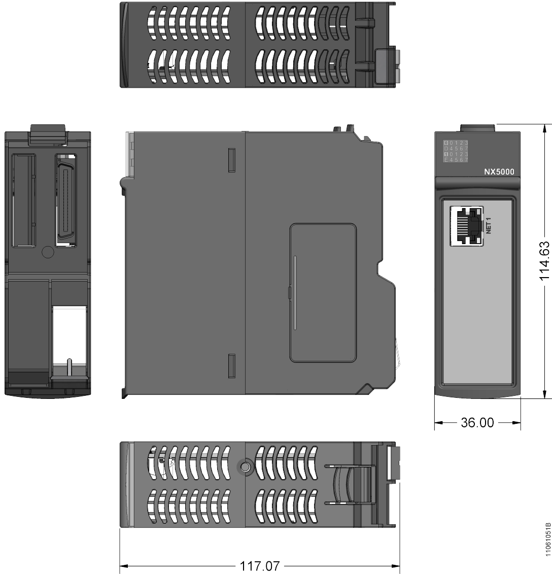
Figure 1: Physical Dimensions
