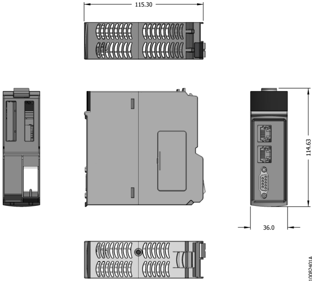
Figure 2: Physical Dimensions
