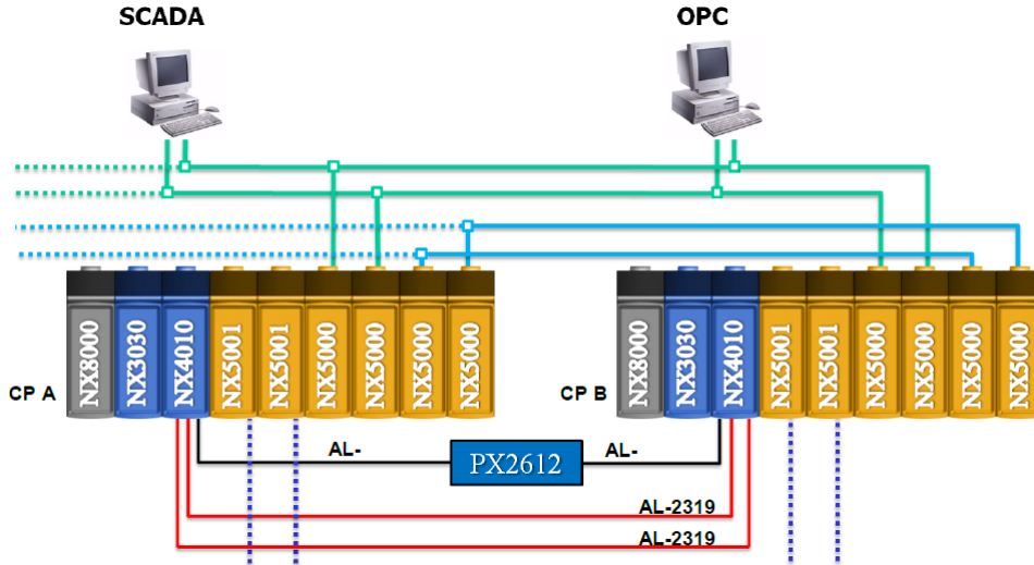
Figure 1: System Configurations
