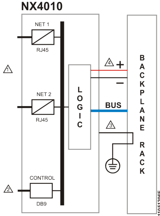
Figure 4: Electrical Installation
