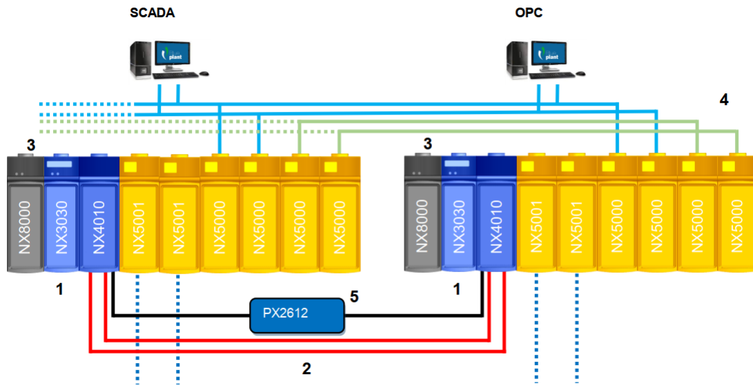
Figure 1: Half-Cluster Redundancy
