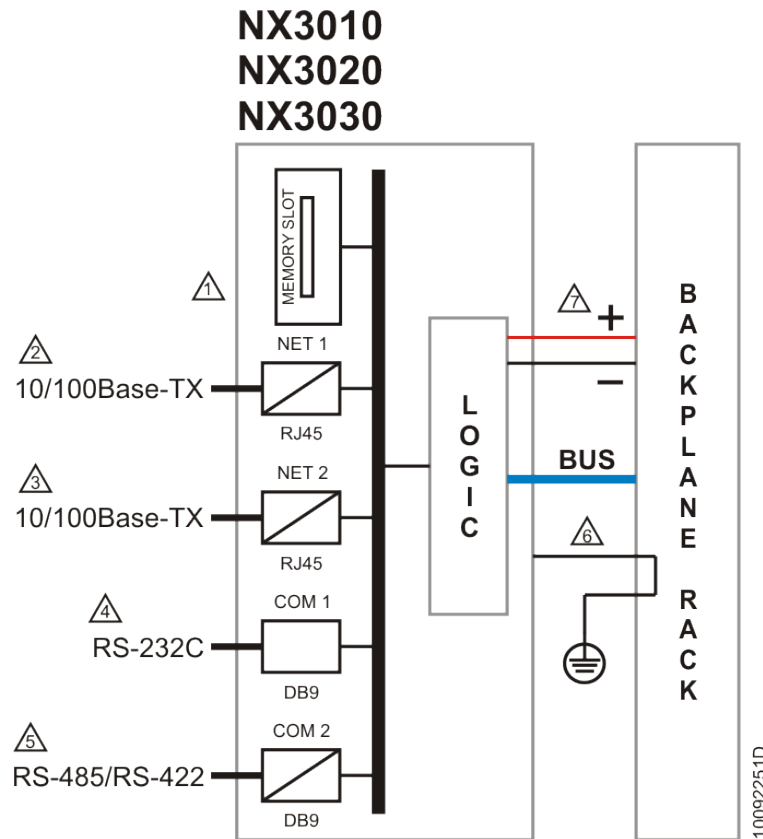
Figure 3: Electrical Diagram of Nexto Series NX3010, NX3020 and NX3030 CPUs
