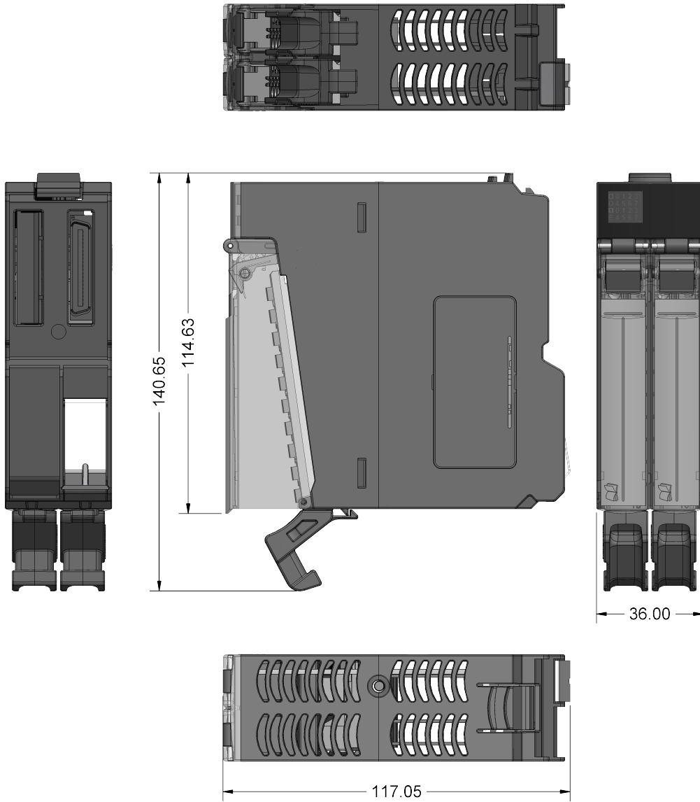
Figure 1: Physical Dimensions
