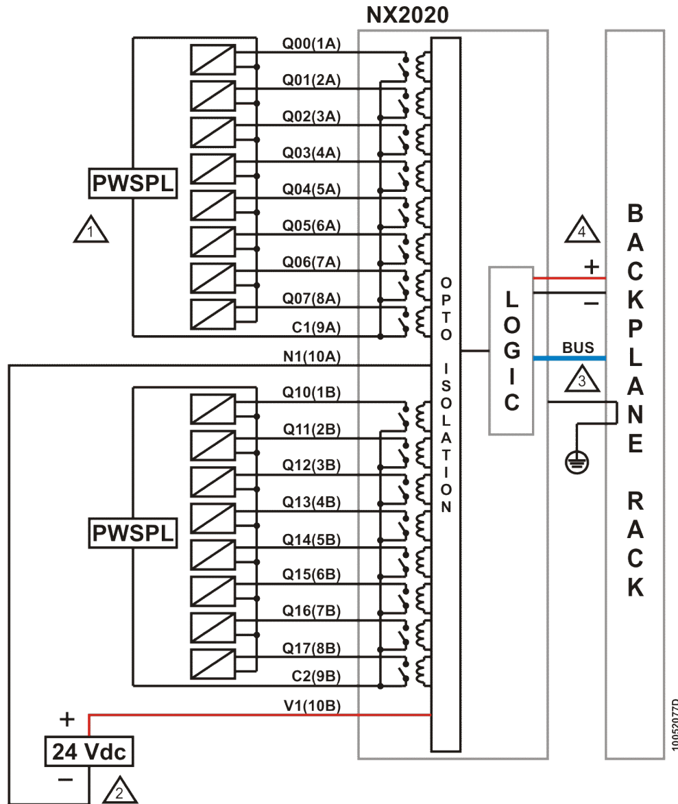
Figure 3: Electric Diagram
