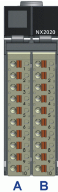
Figure 4: Connector Pinout
