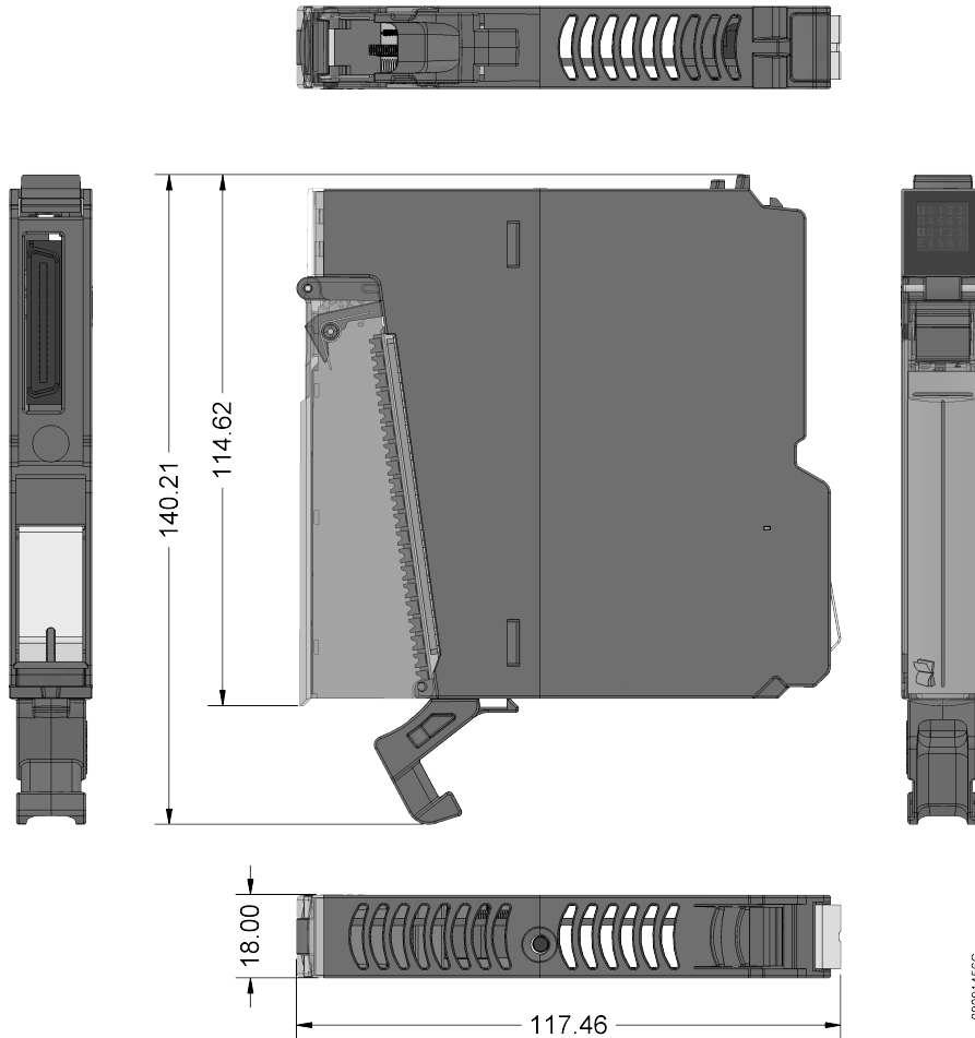
Figure 1: Physical Dimensions
