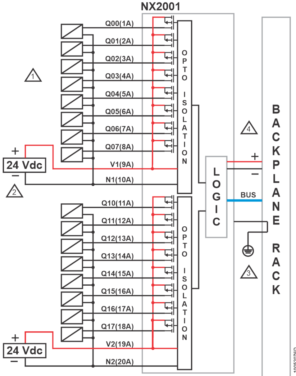
Figure 3: Electric Diagram
