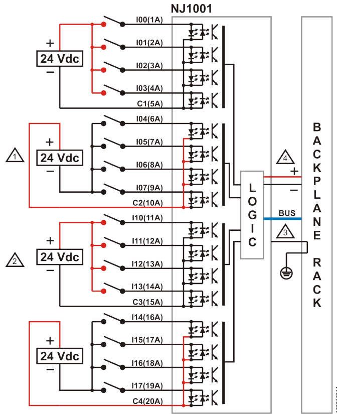
Figure 3: Electric Diagram
