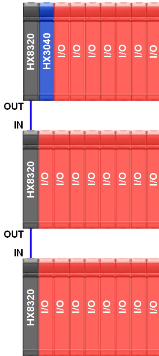
Figure 2: Bus Expansion without Loopback
