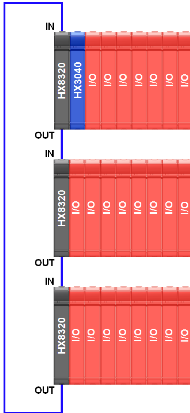
Figure 3: Bus Expansion with Loopback
